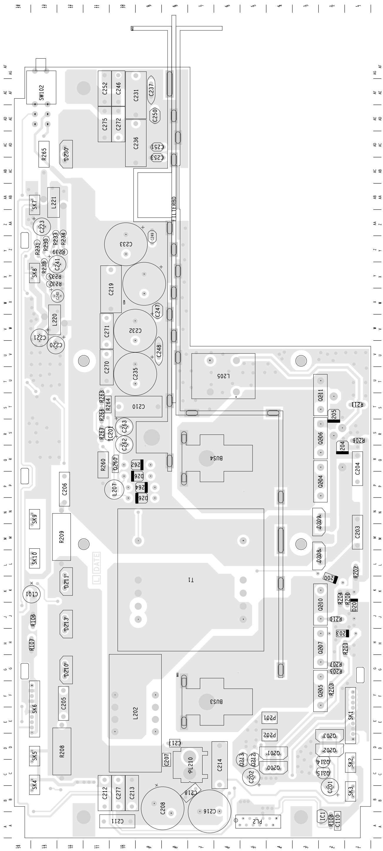
TAIT ELECTRONICS 220-02050-03 A 2006v05 ANTIS TB8000-48V DC-DC CONVERTER LAYOUT-PRIMARY-SIDE
